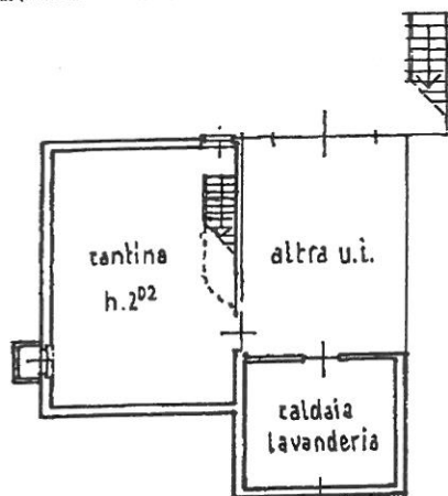
PIANO INTERRATO
